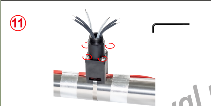
11: Compress the seal by screwing the upper part of the foot with the 4 screws until the both parts are in touch.
