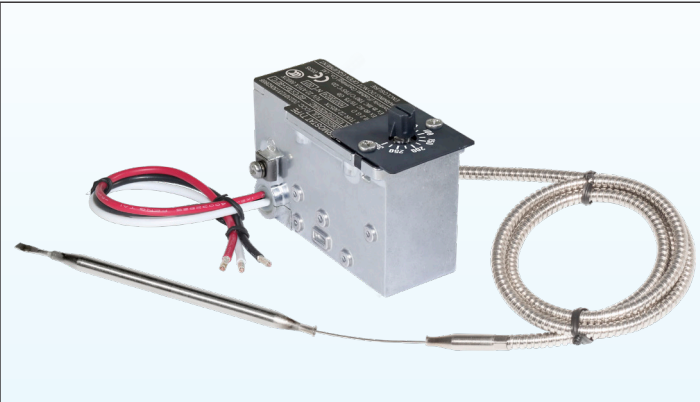
Thermostat type KAA with miniature knob 66MQ and 66CP02 printed dial
