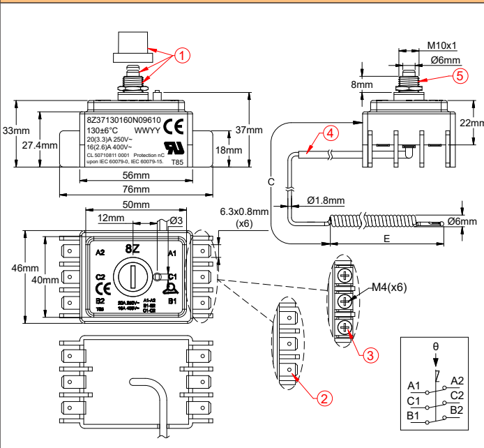
Mounting by M10×1 front bushing or mounting brackets, horizontal terminals, type 8Z31 and 8Z37
