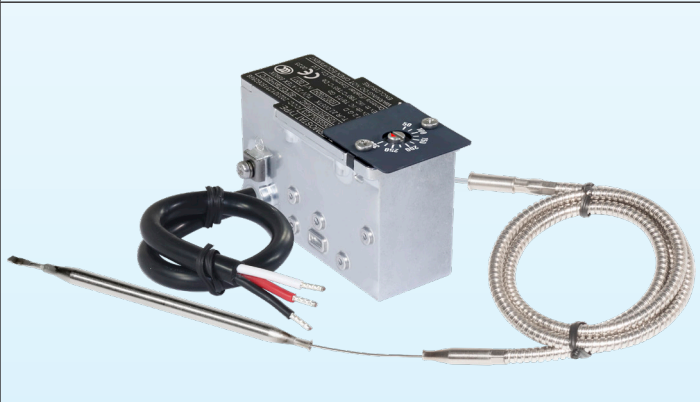
Thermostat type KAC with 66CP01 printed dial assembled with 2 screws M4
