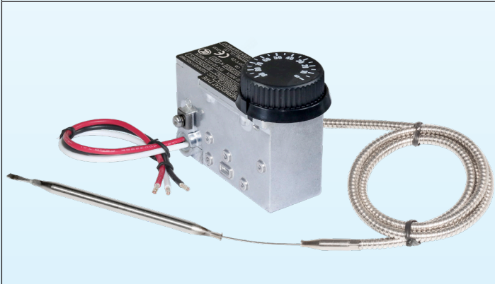
Thermostat type KAA with adjustable stop knob 66ME and 66EN1 bezel
