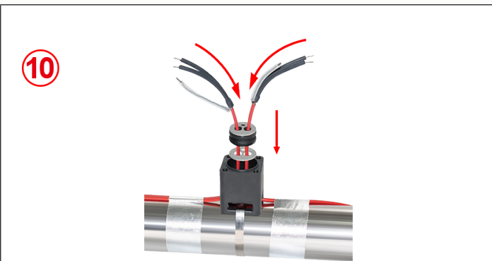
10: Fill the mouth of the silicone boot with silicone resin (RTV). Slide the boot over the conductors of the heating cables, leaving the earth conductor outside. Then slide the ground wires protection sleeves. These boots can also be replaced by a heat-shrinkable tube.
