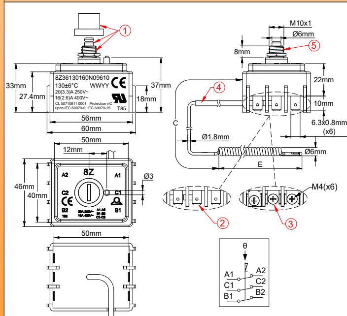
Mounting by M10×1 front bushing, vertical terminals (standard), type 8Z30 and 8Z36
